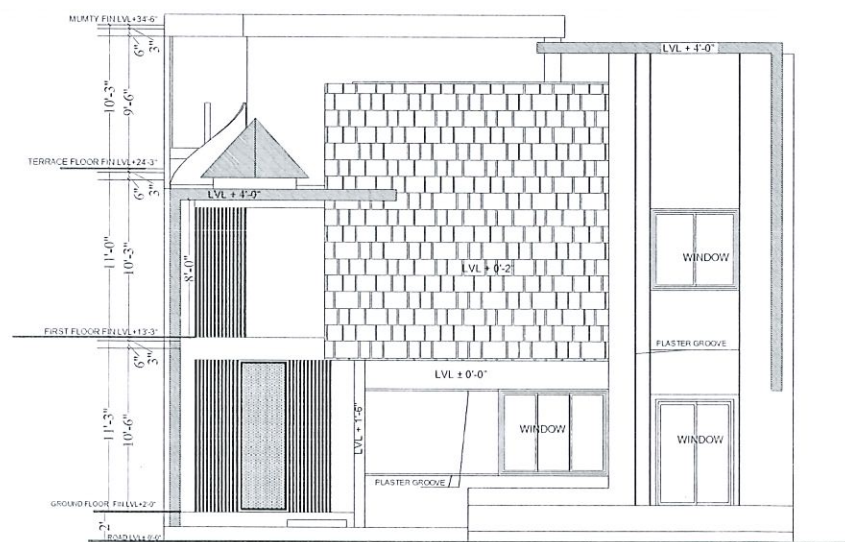
FRONT ELEVATION
